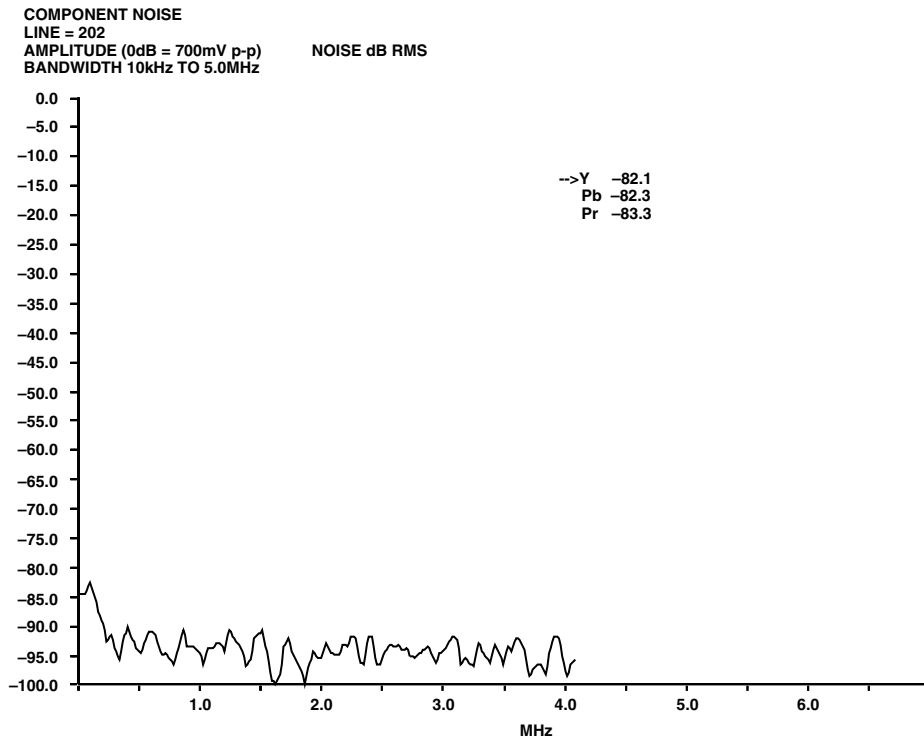
Figure 99. PAL YUV SNR Plot
